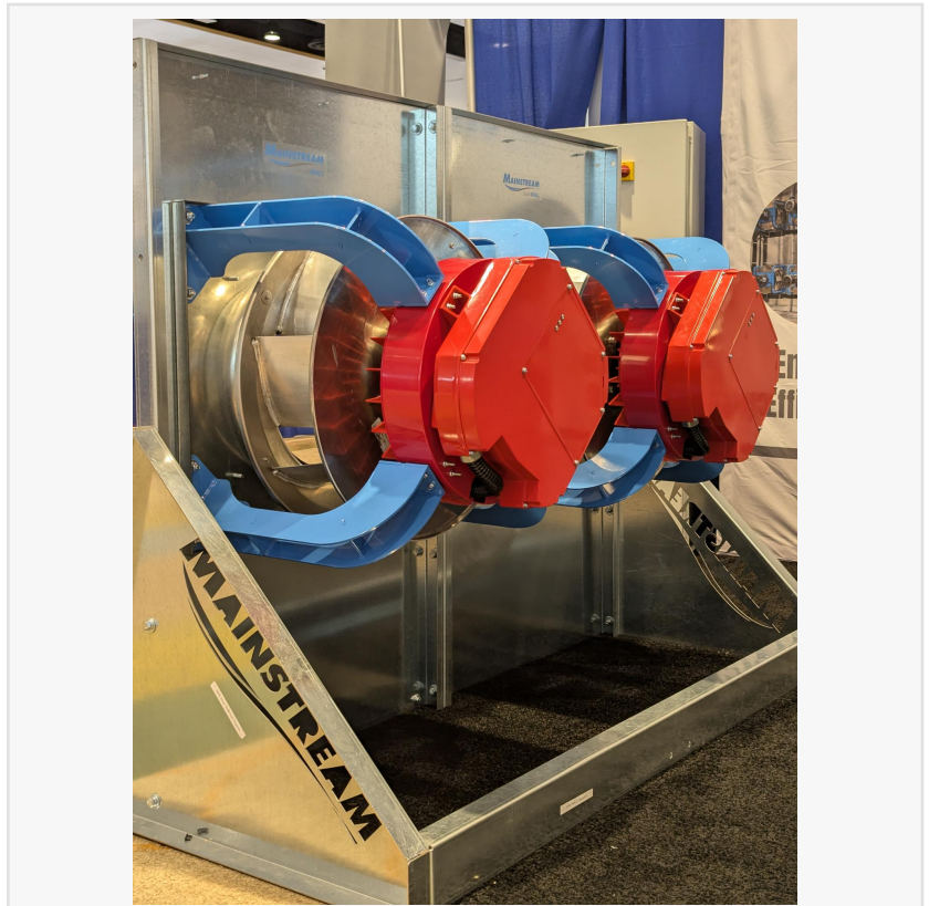
IntelliWALL with Infinitum EC Motor
