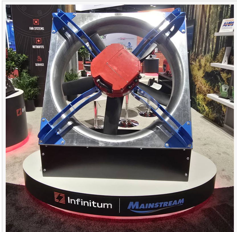
Mainstream EDA Axial Fan with Infinitum EC Motor
