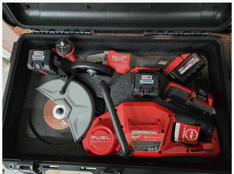
MILWAUKEE BREACHING SAW KIT BY DEVOUR 9 INCH SAW AND 5 INCH GRINDER
