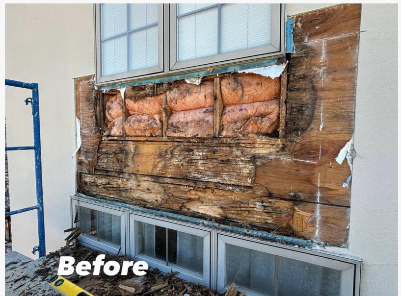
Open stucco system - before
