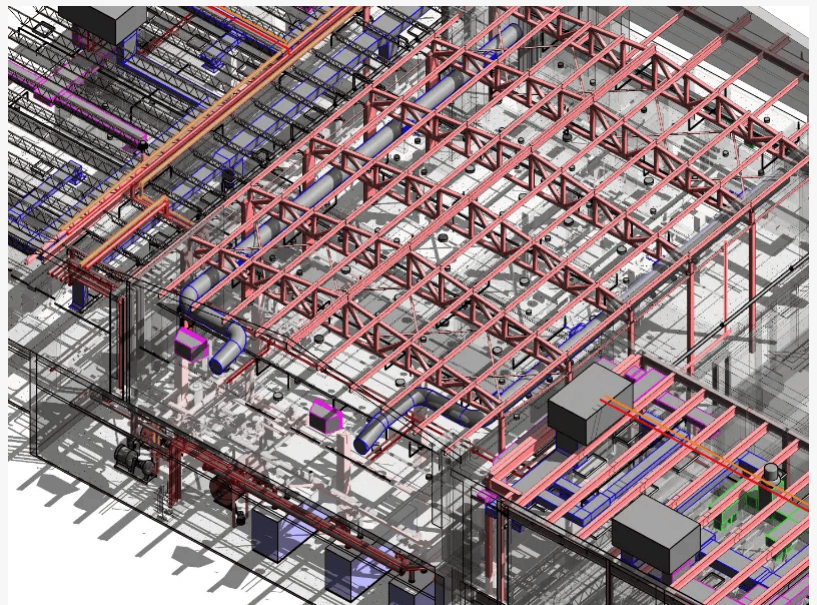
LOD 350 MEPF BIM Coordination Model of Commercial Complex
