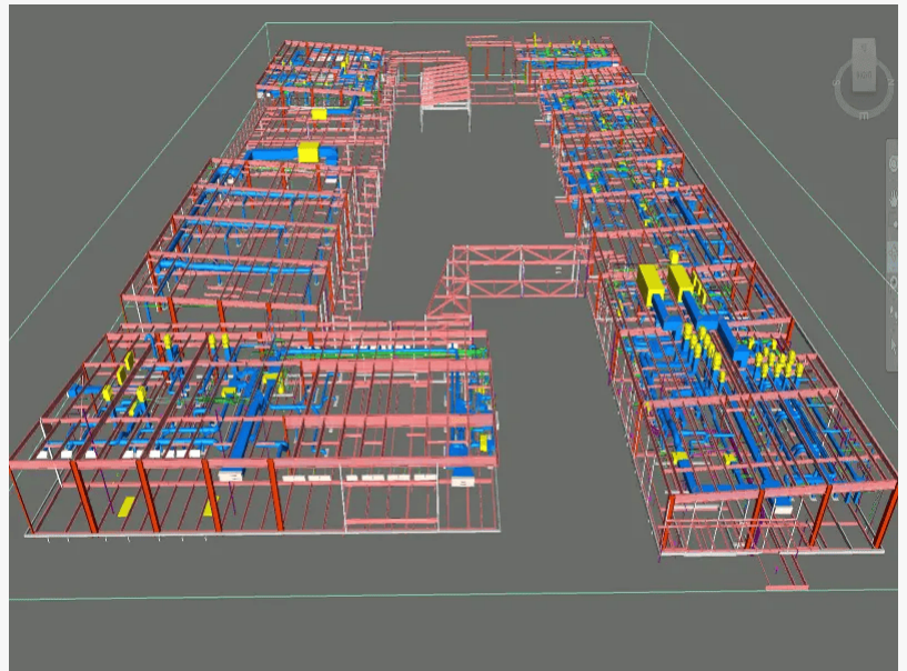
Multidisciplinary Structural MEP BIM Coordinated Model
