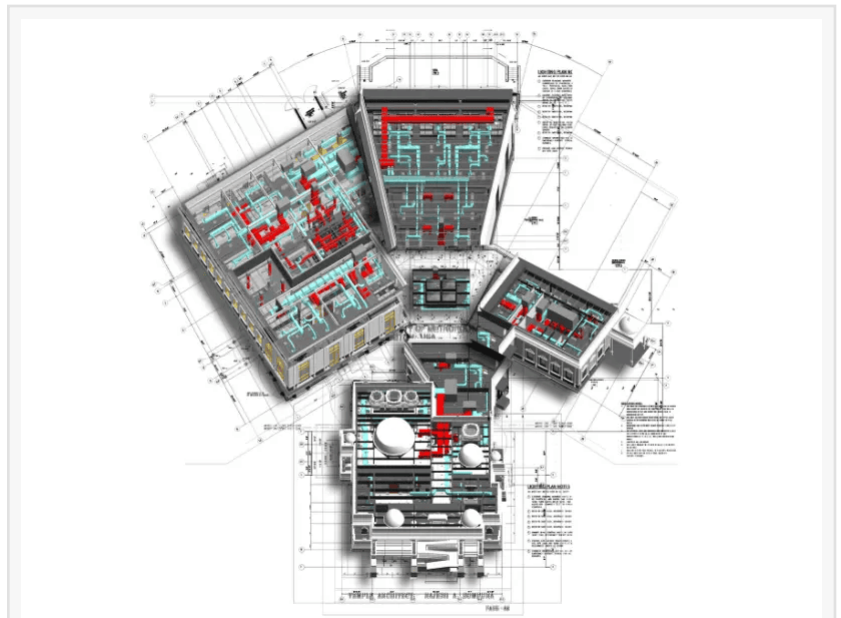
MEP Coordination Model of Religious Building
