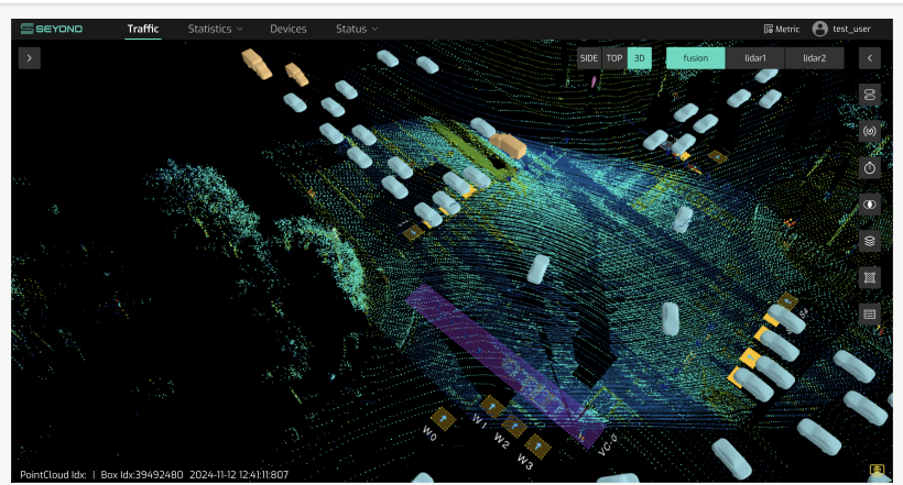
Detecting road users in real-time with SIMPL
