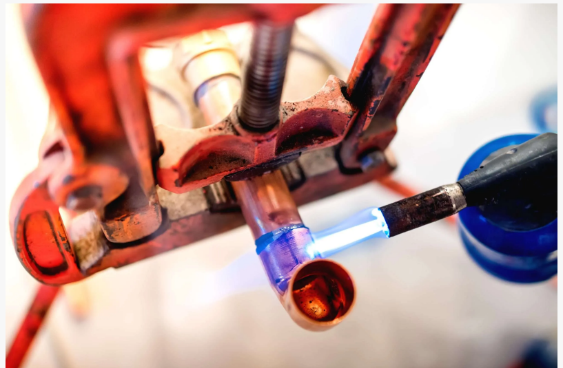
copper pipe pinhole repair
