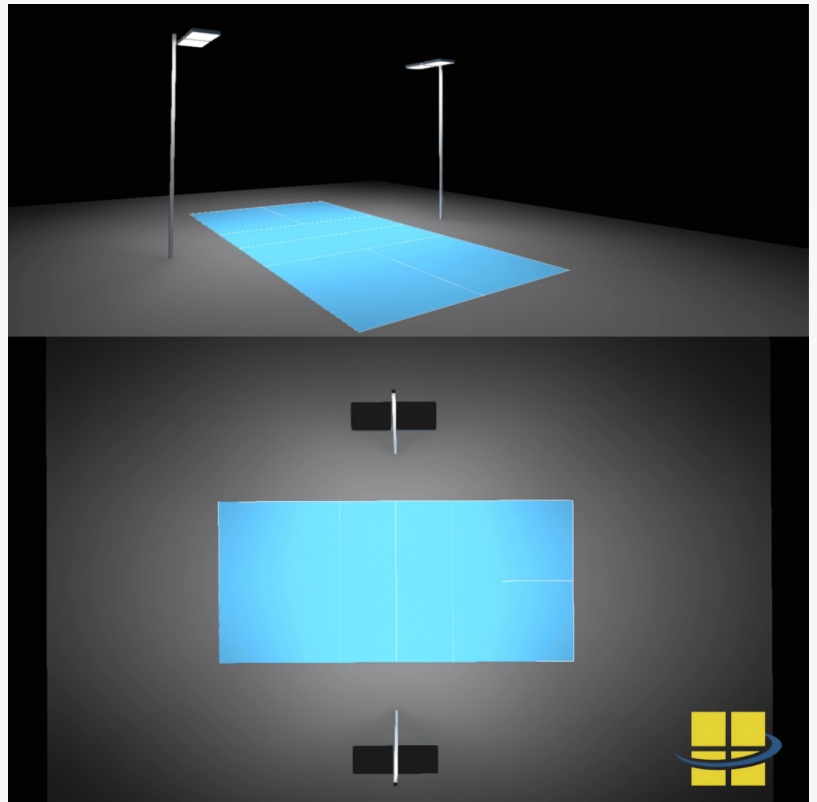
Pickleball Single Court Solar LED Lighting
