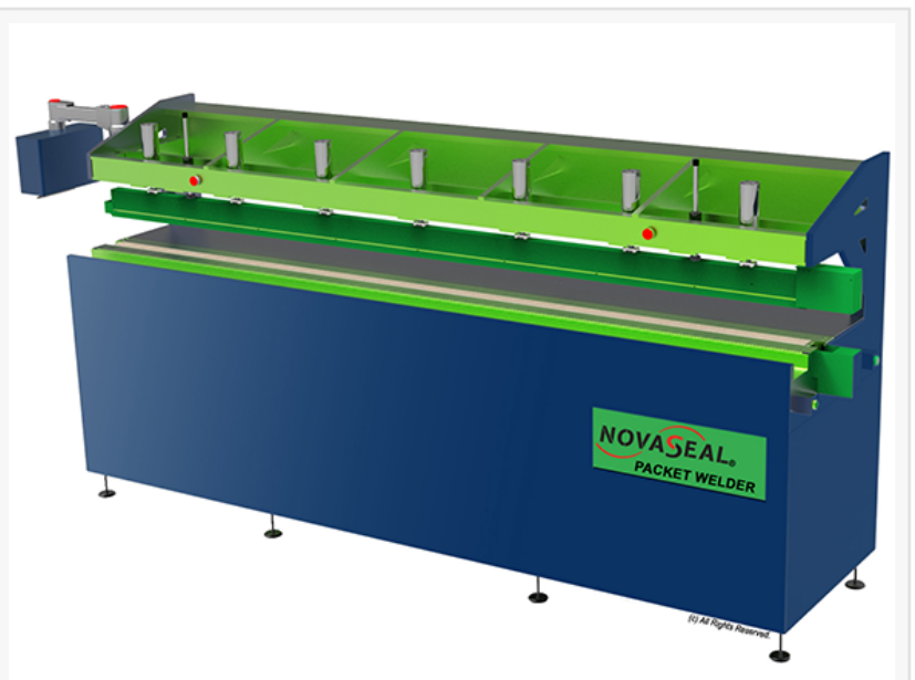
Standard Model
