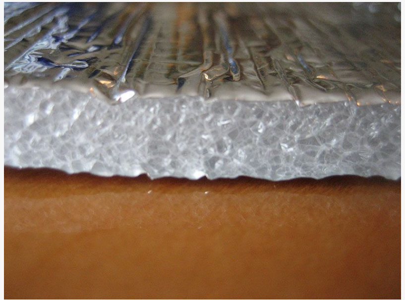
Center of Prodex Total Insulation Roll
