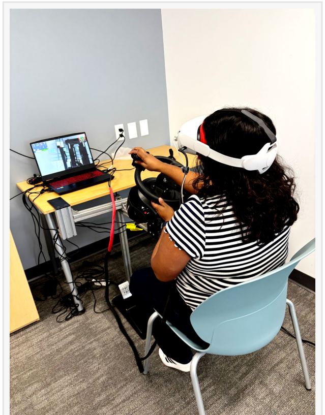
BluWorkz Mobile VR Forklift Simulator
