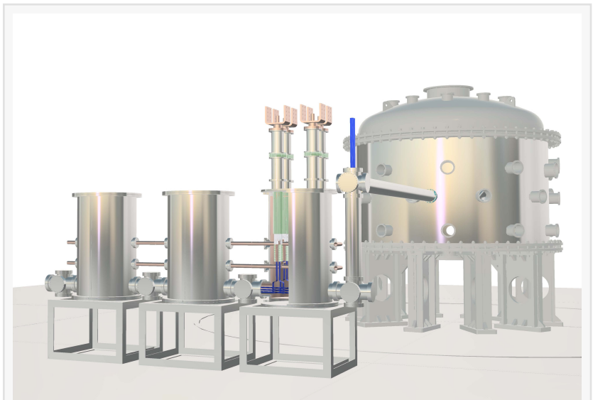
Concept image including a current lead for HTS coils (created by Helical Fusion)
