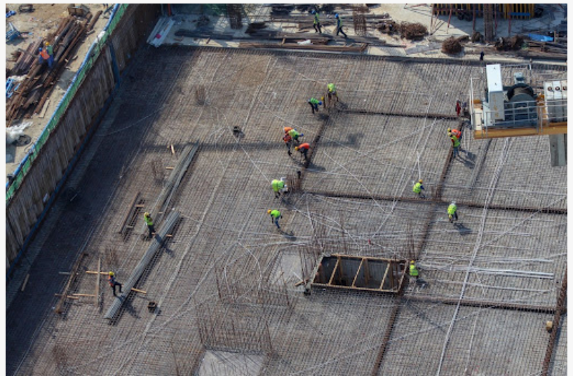
Aerial view of workers installing concrete at an active construction site
