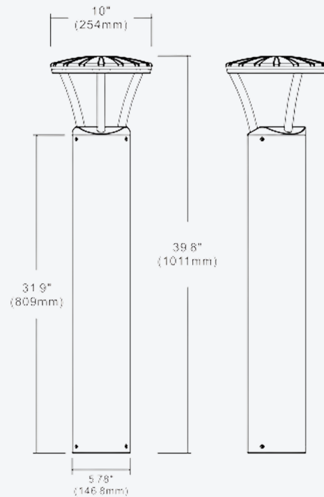
ABUR - Vandal Proof LED Bollard Light (Fixture Dimensions)
