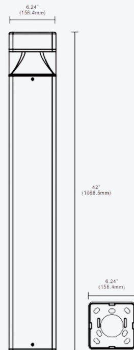
SQUO - Square Heavy Duty LED Bollard Light (Fixture Dimensions)
