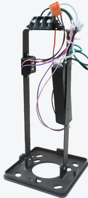
SQUO - Square Heavy Duty LED Bollard Light (Mounting Plate)
