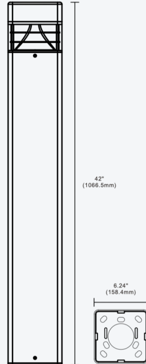
SPOO - Heavy Duty Vandal Proof LED Bollard Light (Fixture Dimensions)
