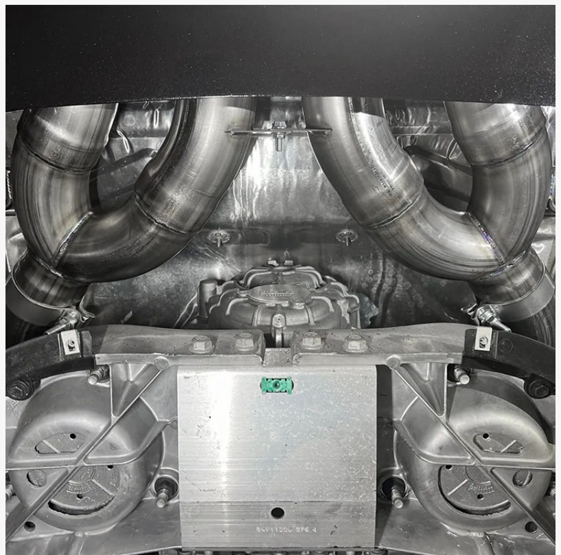
MRT 304 Stainless Cat-back C8 Z06 91S226 - Installed
