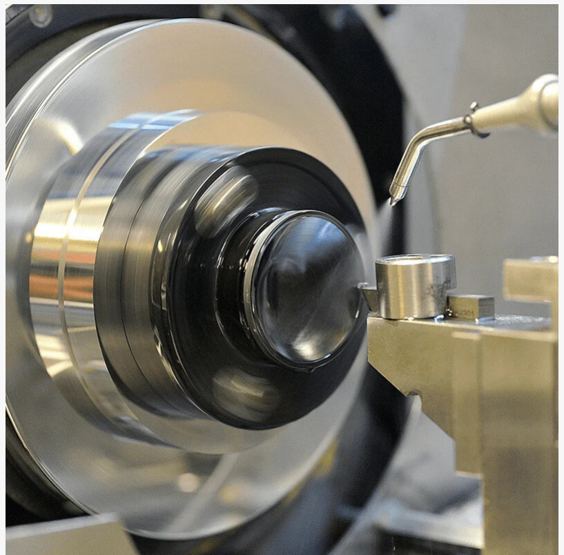
LightPath thermal imaging optics manufacturing
