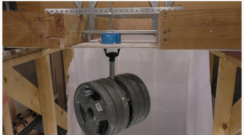
Fixture support system
