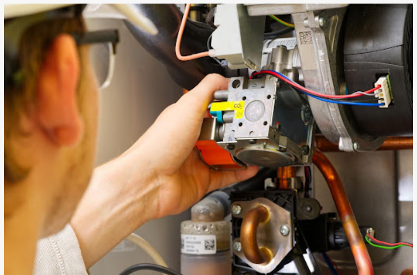
Technician setting up and fine-tuning the boiler system to ensure efficient and reliable heating performance.
