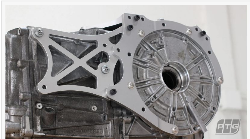
PTG 7DCL750 AMG GT / SLS Billet Transmission Brace System
