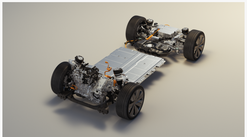
Technical diagram of the 800V active suspension and steer-by-wire chassis
