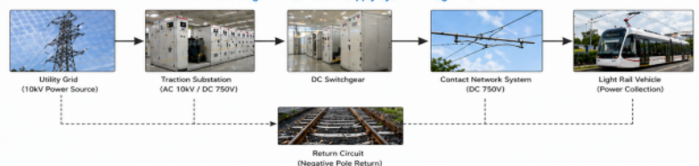
Structure Diagram of DC Power Supply System for Light Rail Transit
