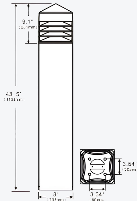
ARCO 40w Square Heavy Duty Vandal Resistant LED Bollard Light (Dimensions)
