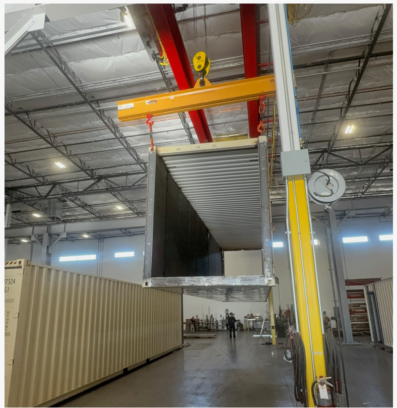
A bridge crane lifting a shooting range container.
