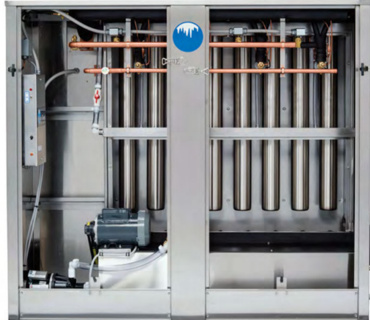
1500 RCU Industrial Ice Machine
