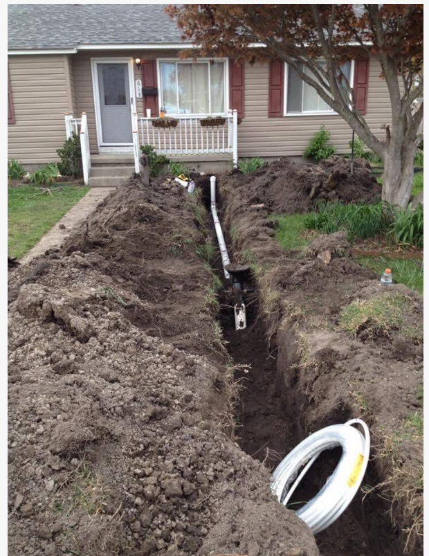
A trenched sewer line installation completed by Newman's Plumbing.
